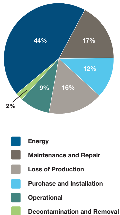
Typical pump lifecycle costs 1
