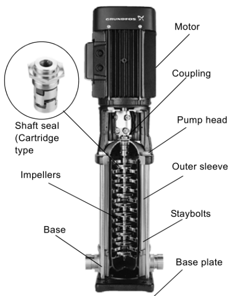
Fig. 3 CR pump
