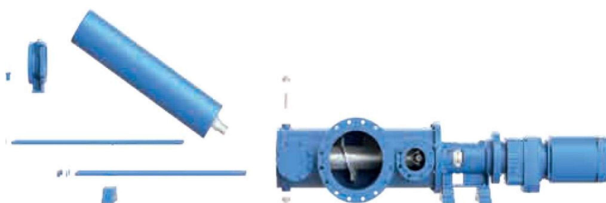
view from the side with opened X-LIFT quick change system
