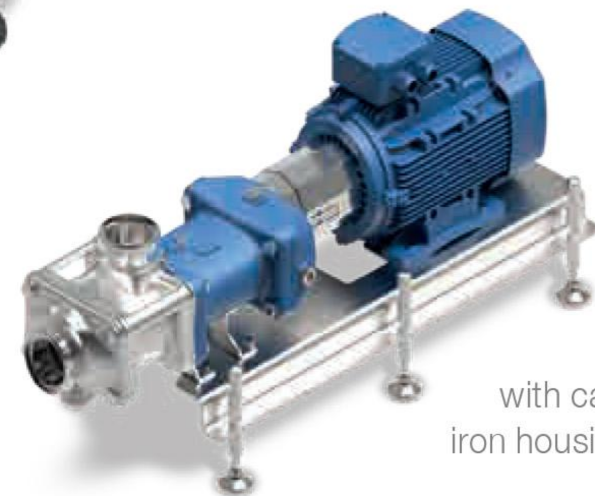
WANGEN Twin 104 NG series with stainless steel housing
