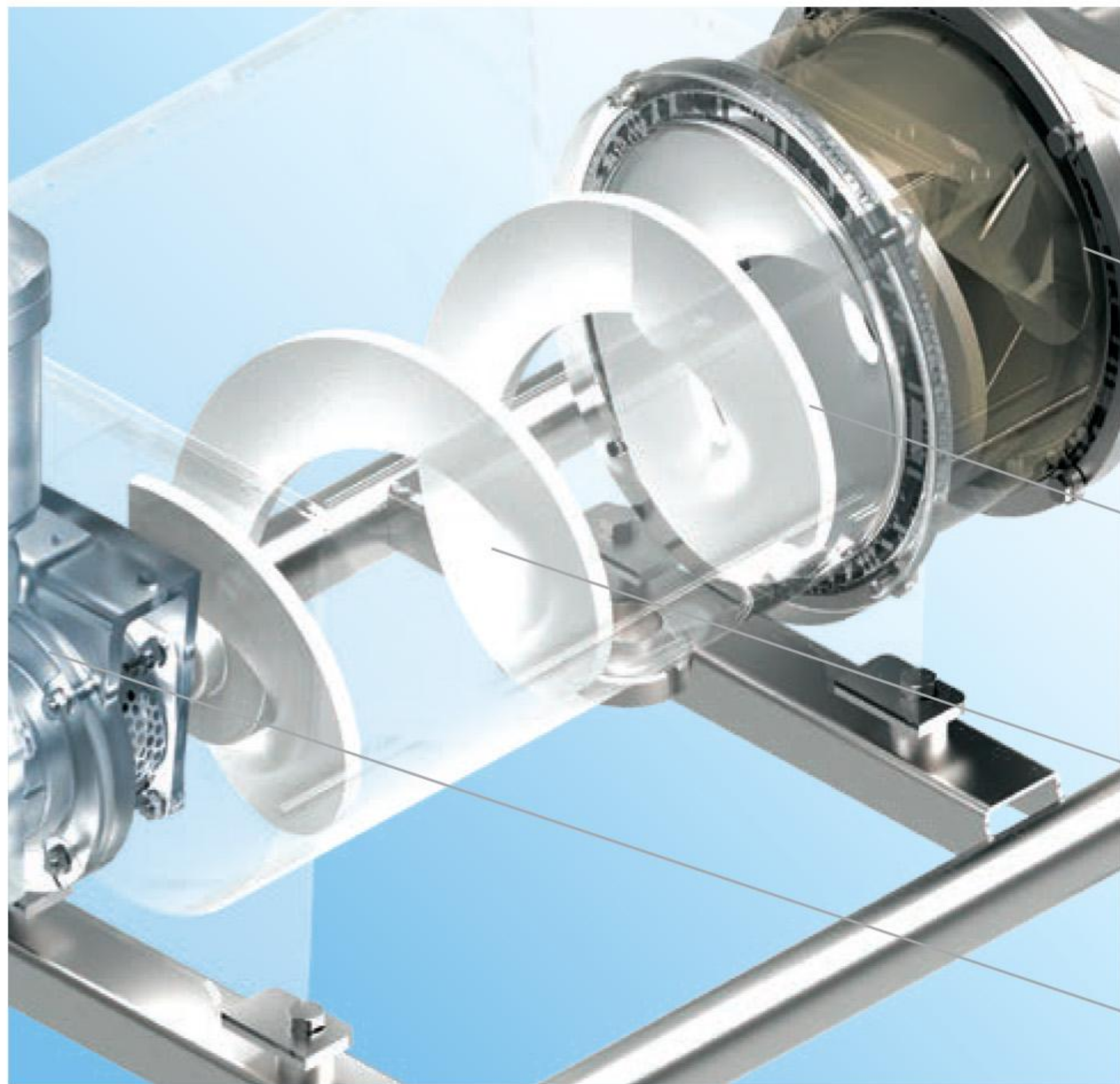
Cross-section of the 'VarioTwin NG' hopper.
